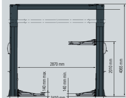
SDH370.42K VAR WIDE SDH370.45KEX VAR WIDE
